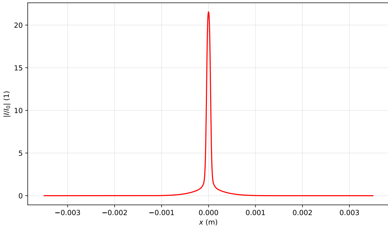
Intensity profile I(x, y = 0, z = 0.478)/I_0 , P_{in}=5.0P_{cr} , artificial time
